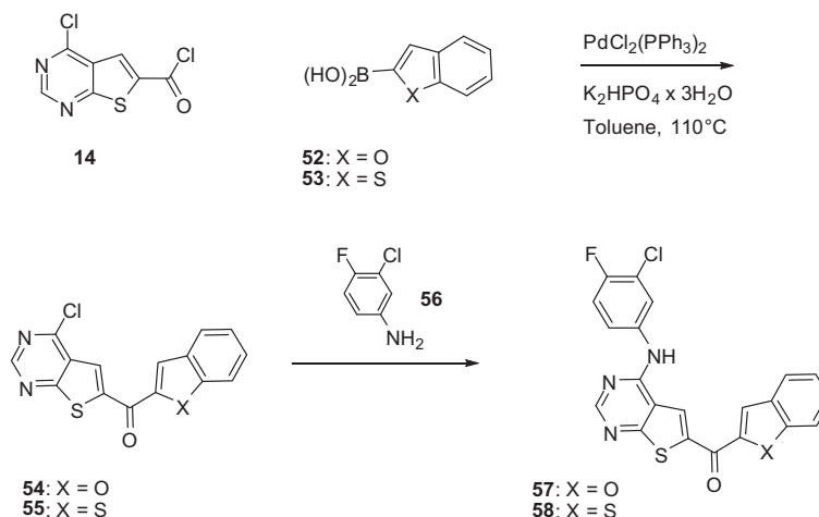
Scheme 2. Synthesis of 57 and 58 , respectively.
