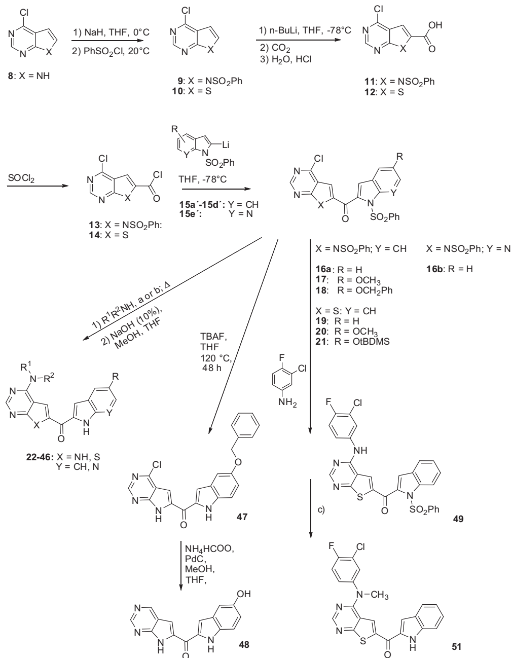
Scheme 1. Synthetic path for preparation of (4-(arylamino)-7H-pyrrolo[2,3-d]pyrimidin-6-yl)(1H-indol-2-yl)methanones and (1H-indol-2-yl)(4-(phenylamino)thieno[2,3-d]pyrimidin-6-yl)methanones. For definitions of X, R, R 1 and R 2 see Tables 1 and 2. Conditions: (a) 2-butanone, 2 d; (b) n -butanol, 12 h; (c) (1) NaH, THF, CH 3 I, (2) NaOH (10%), MeOH, THF. Formulas for 15a'–15e' show the lithiated species corresponding to indole-derivatives 15a–15e .
