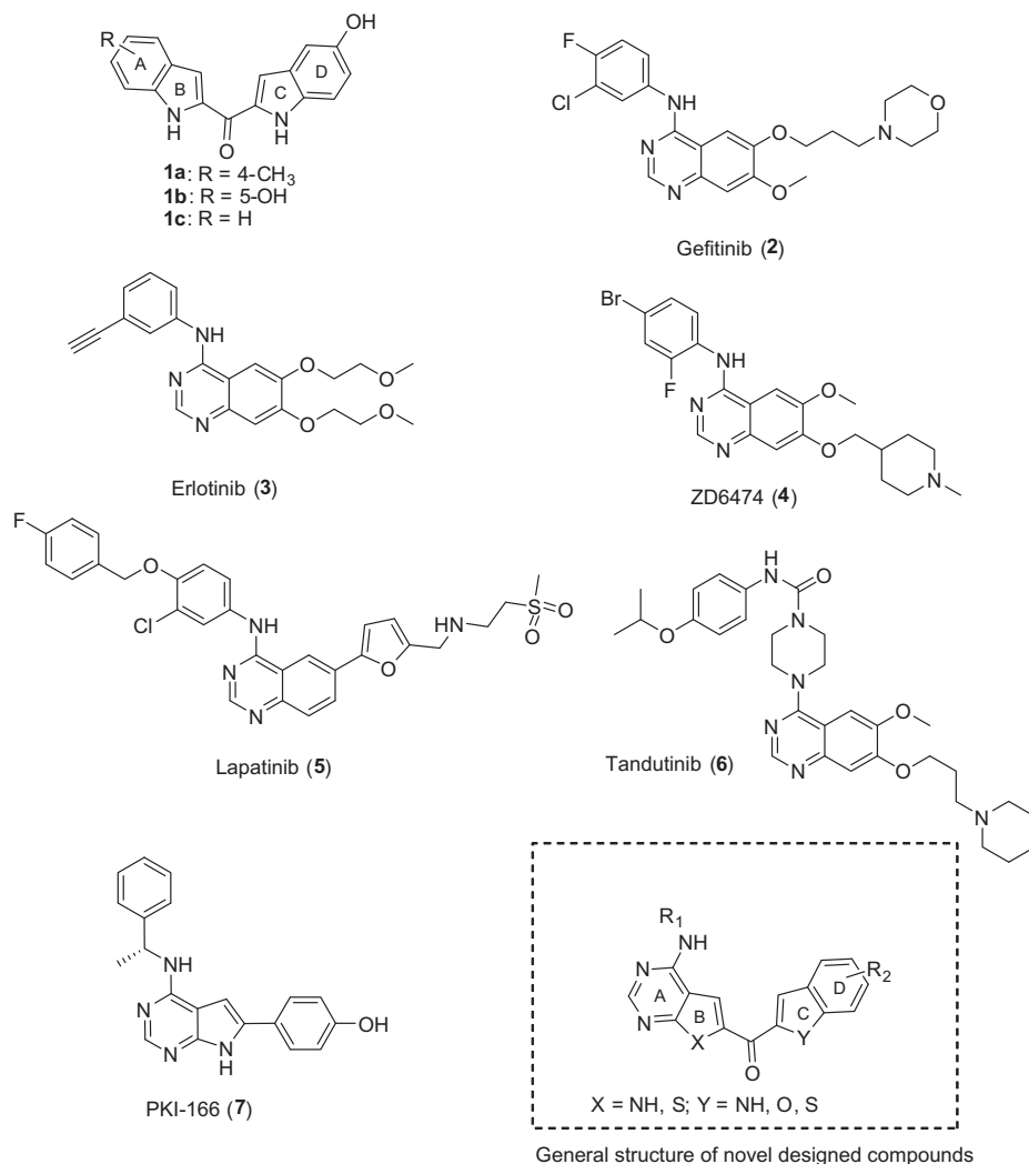
Figure 1. Structures of 2-indolylmethanones (e.g., 1a and 1b ), well known tyrosine kinase inhibitors containing the pyrimidine core structure as part of a quinazoline system, and general structure of newly designed compounds.
